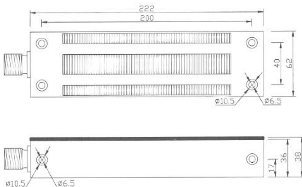
Magnetic lock dimension drawing
